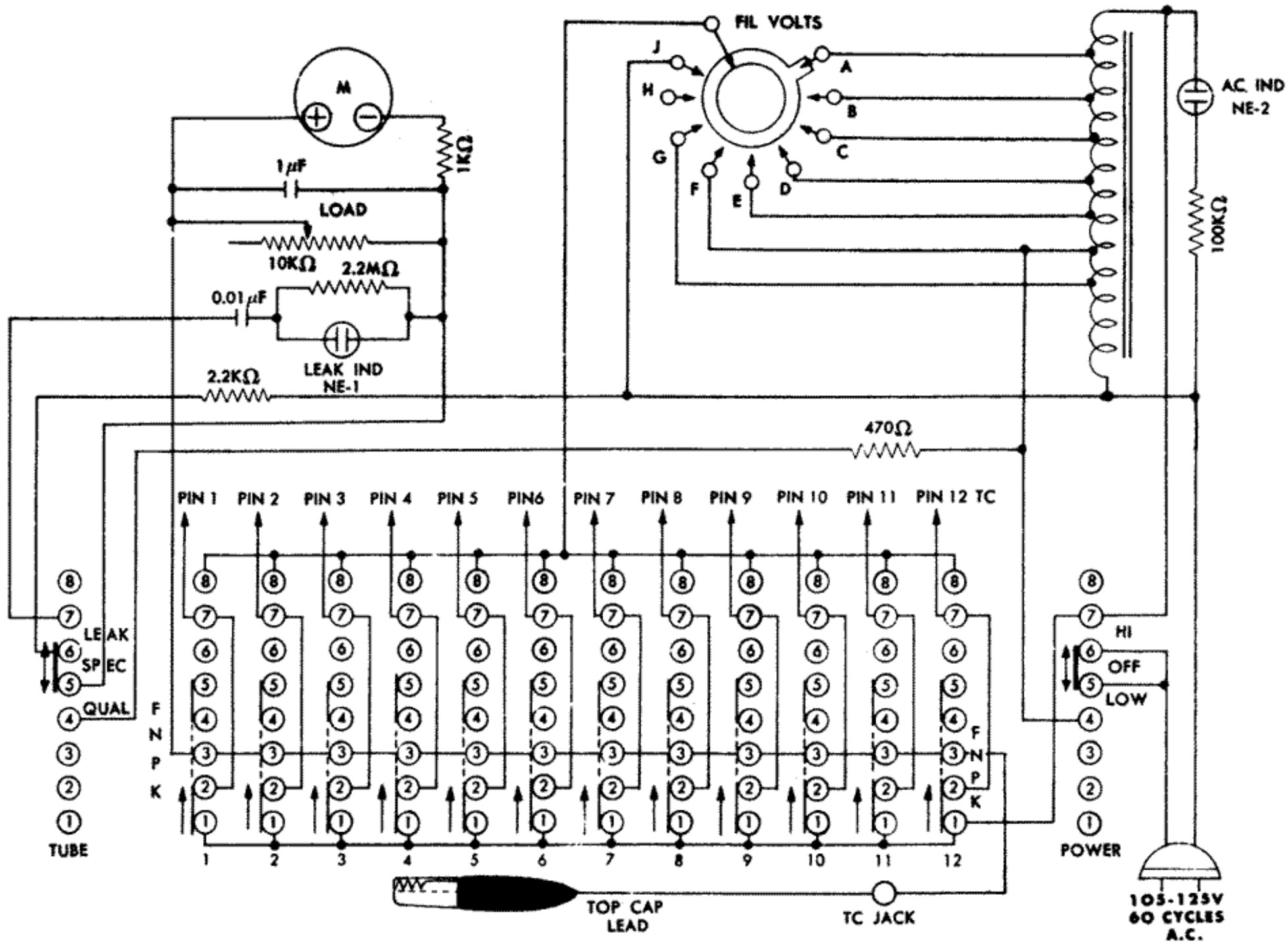
SCHEMATIC DIAGRAM
